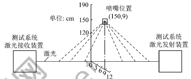
Fig. 1 Experimental system of nozzle spraying
